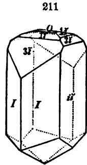
Calamine.
